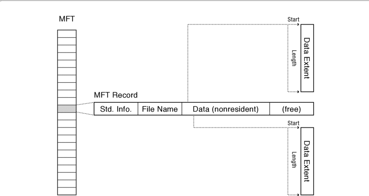
Figure 13.15: NTFS index structures and data for a basic file with two data extents.
