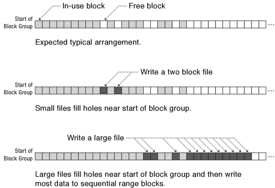
Figure 13.14: FFS's block placement heuristic is to put each new file block in the first free block in that file's block group
